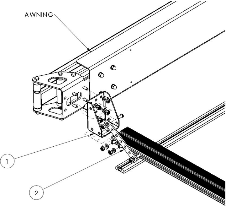
TYPICAL FITTING POSITION OF AWNING BRACKET
