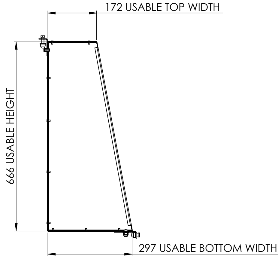
SECTION B-B
