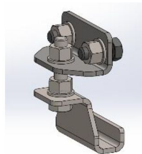
Figure 10: Centre Mounting Bracket Assembly
