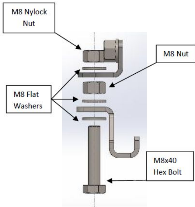
Figure 9: Centre Bracket Mounting Assembly
