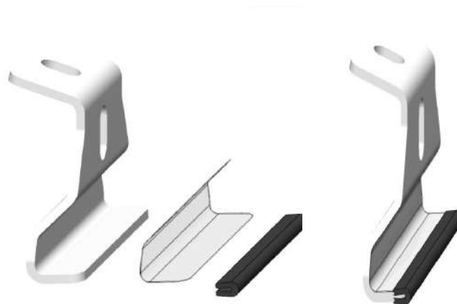
Figure 4: Tension Plate with 3mm rubber channel
