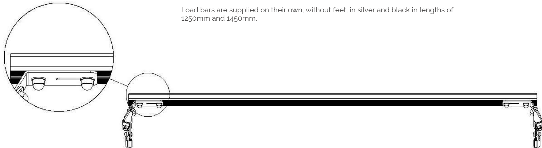
Figure 5: Load bar mounting to Top Plate
